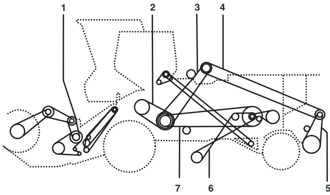
WITH REAPER AND SHREDDER
