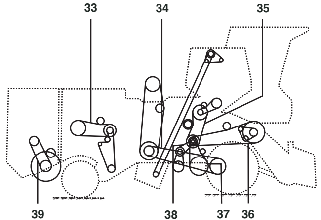
WITH MECHANICAL DRIVE UNDERCARRIAGE AND SHREDDER
