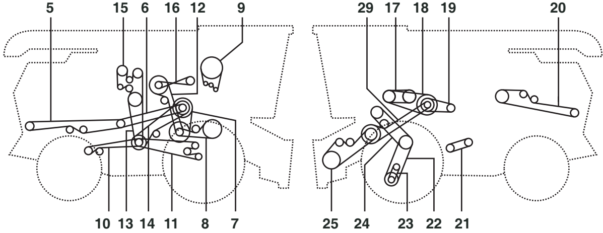
Engine
